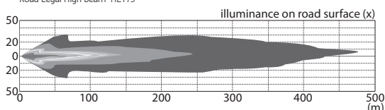
Road Legal High Beam HL175
